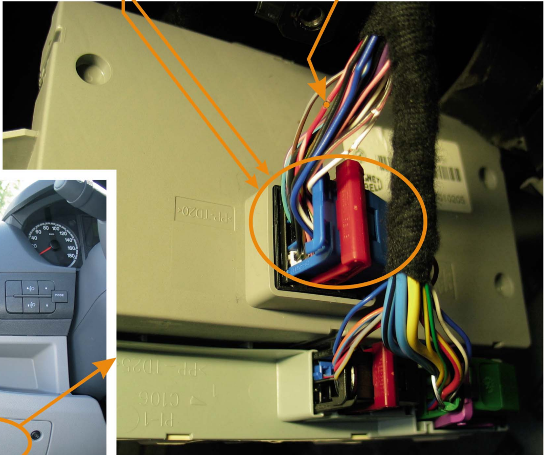
CONTROLLER MODULE (BACK)
