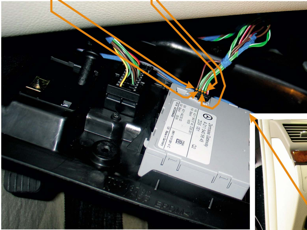
GATEWAY CONTROLLER (above driver's legs)
