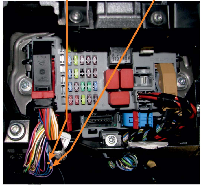
CONTROLLER MODULE (FRONT)
