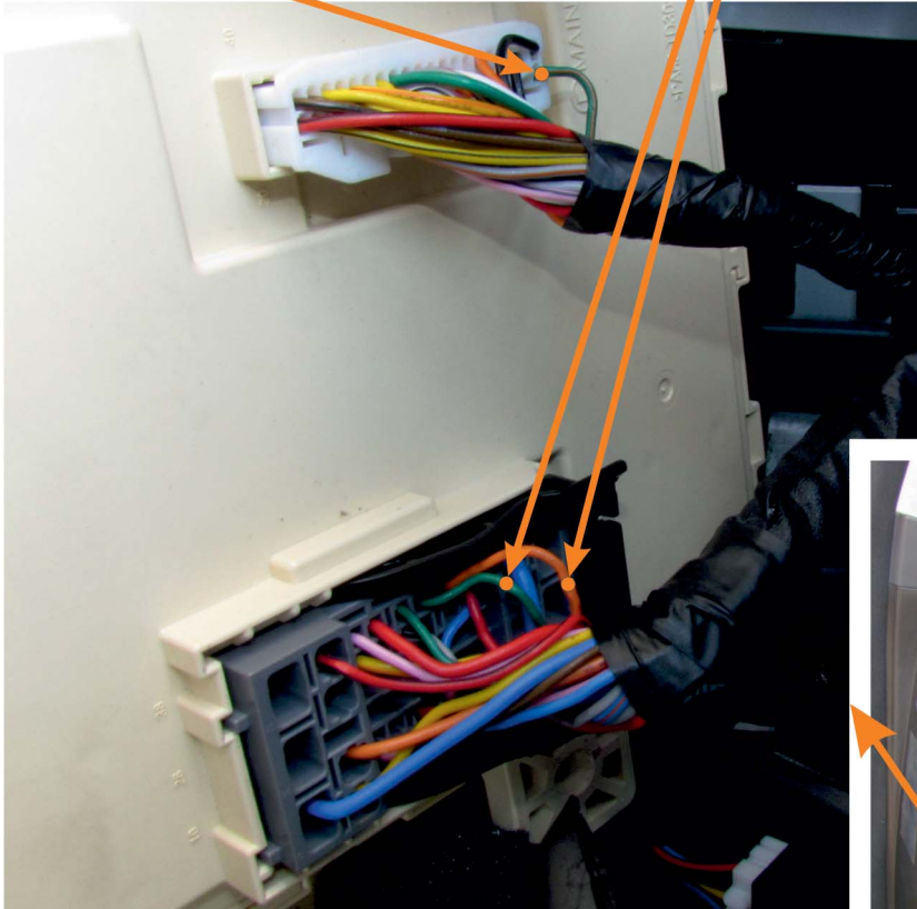
CONTROL MODULE (REAR)
