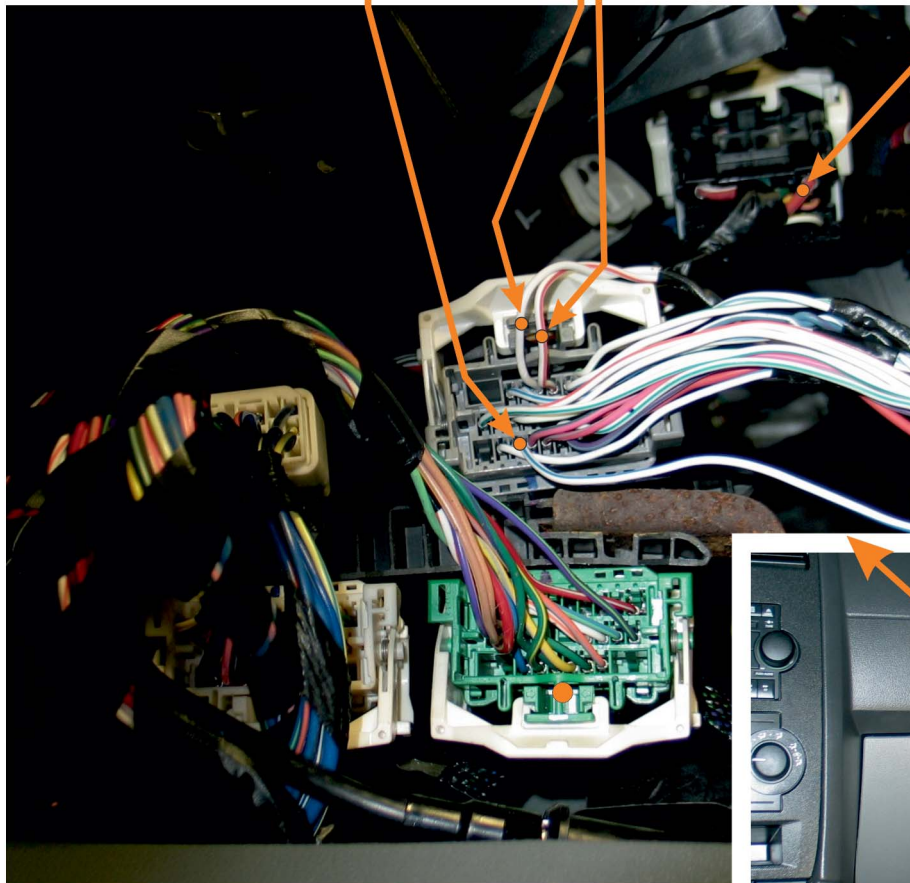
CONNECTORS BEHIND GLOVE COMPARTMENT
